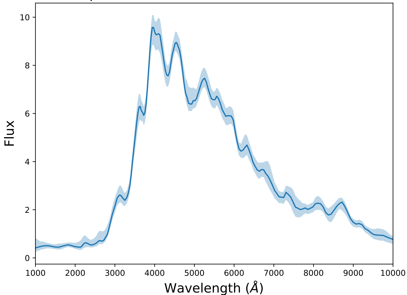
Spectrum 8 for transient SNIax at z=1.45
